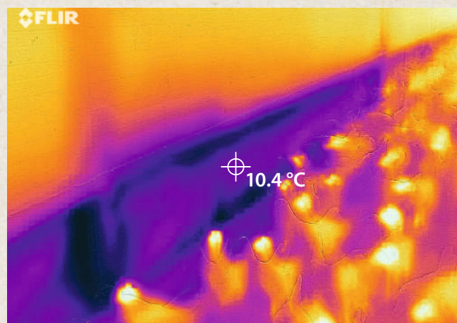
As you see in the infrared image, Pop-holes present a big challenge when trying to keep an optimal temperature and good litter characteristic in the area near them.
