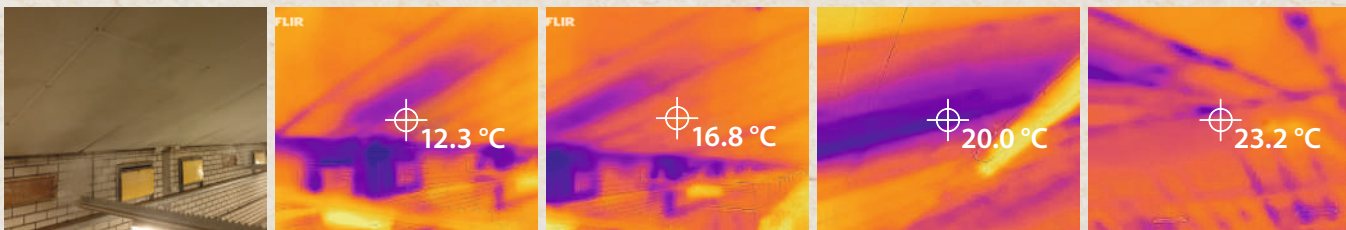
A good transverse ventilation system is intended to warm up the incoming air by directing it to the roof where the air temperature is higher. This sequence of thermal images is showing us the effect of an optimal transverse ventilation
