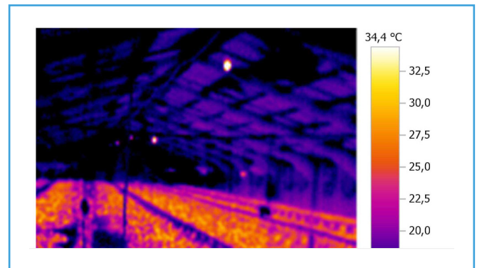
Roof insulation is the corner stone for a correct house temperature and ventilation in hot or cold weather. Courtesy of M. Czarick – UGA
