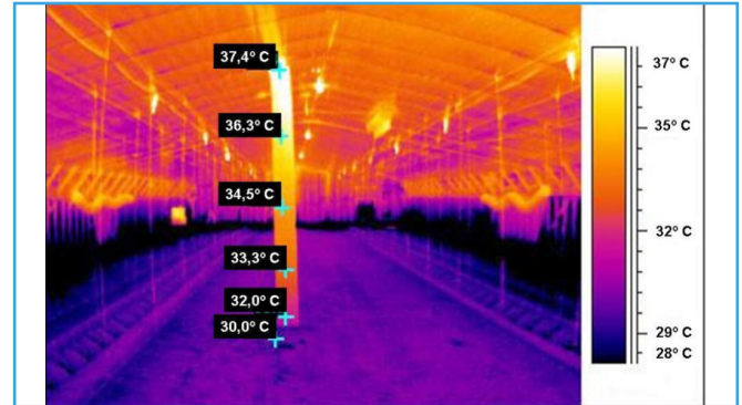
Temperature always has a height gradient. Careful consideration should be taken in cage systems. Courtesy of M. Czarick – UGA
