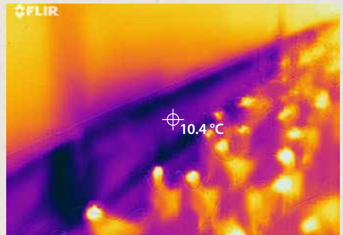
As you see in the infrared image, Pop-holes present a big challenge when trying to keep an optimal temperature and good litter characteristic in the area near them.
