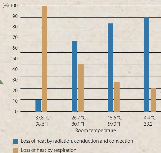
Effects of the Barn Temperature on Heat Loss
