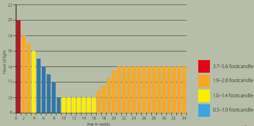
Example of lighting program for dark houses
